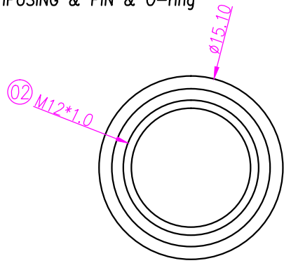
NUT & anti-vibration detent
