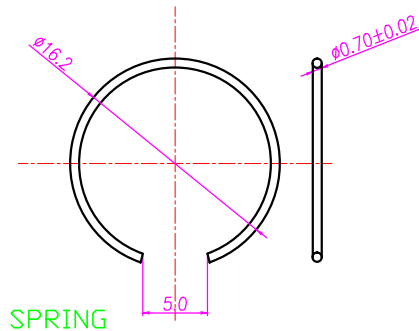
SPRING
